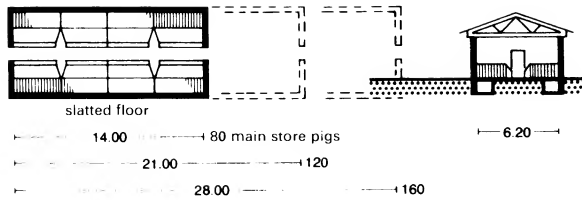
① Store pig shed: two rows, short stalls, longitudinal troughs (80–160 animals)
